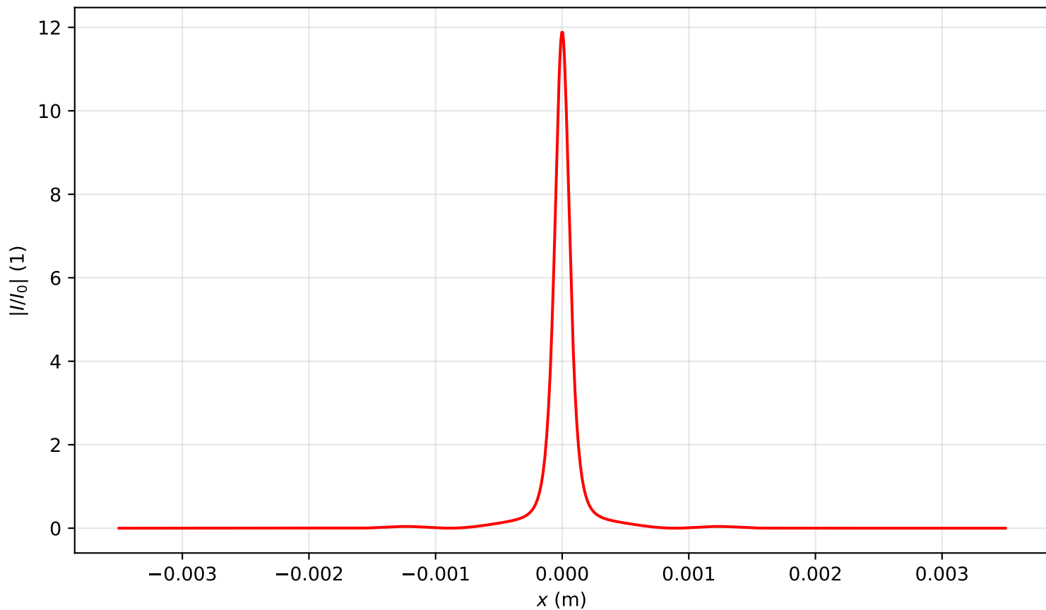
Intensity profile I(x, y = 0, z = 1.911)/I_0 , P_{in}=2.5P_{cr} , artificial time
